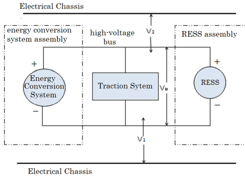
Figure 1: (Measurements of V_b , V_1 , and V_2 )
