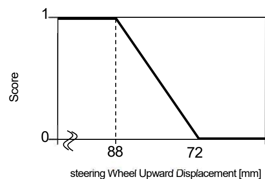
[Fig. 2: Degree of steering Wheel Upward Displacement]
