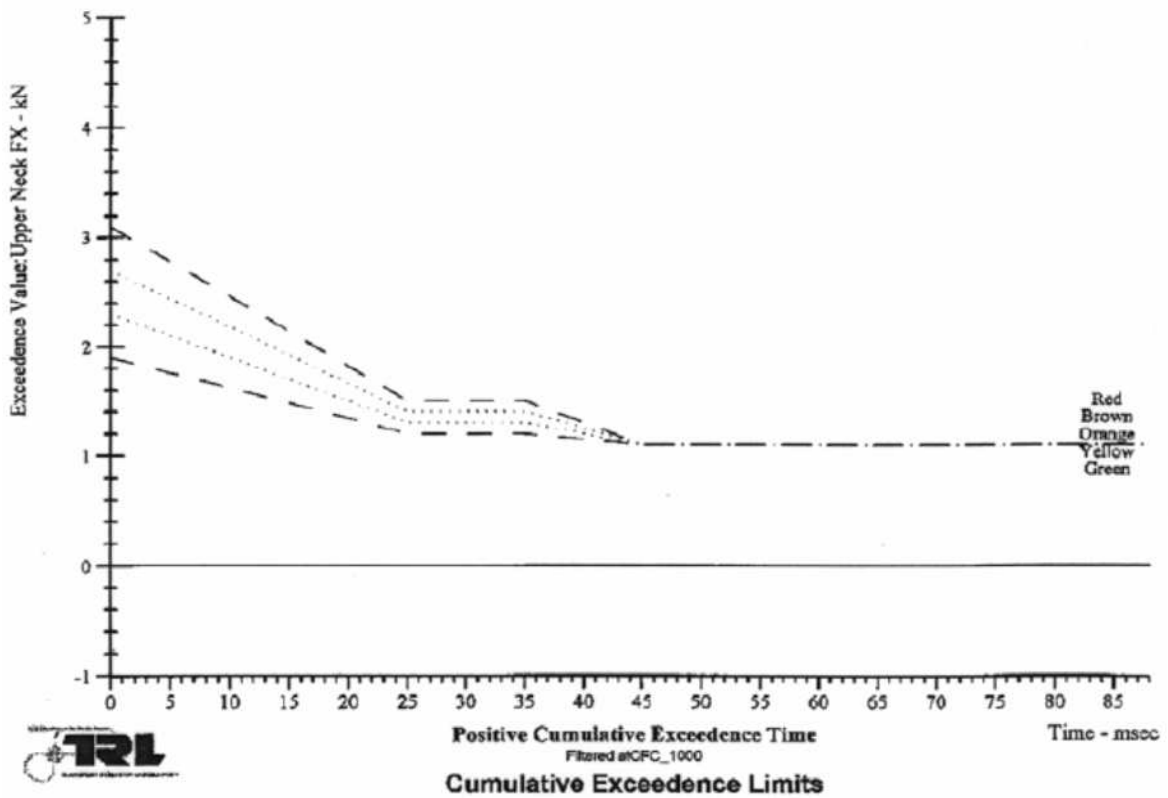
[Fig. 3-2-1: Shearing Load (1)]
