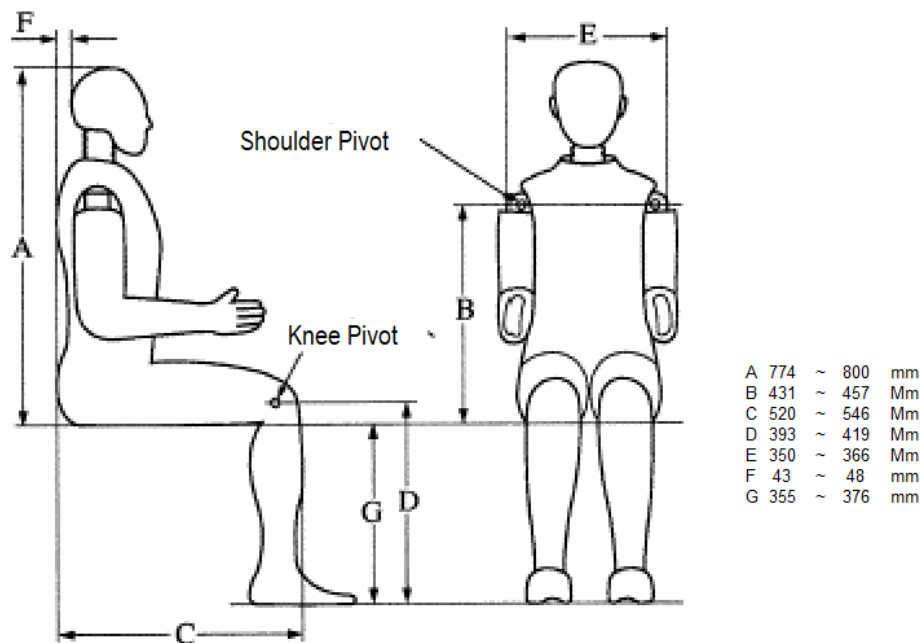
Figure 1: Constructional Dimensions of Hybrid III
