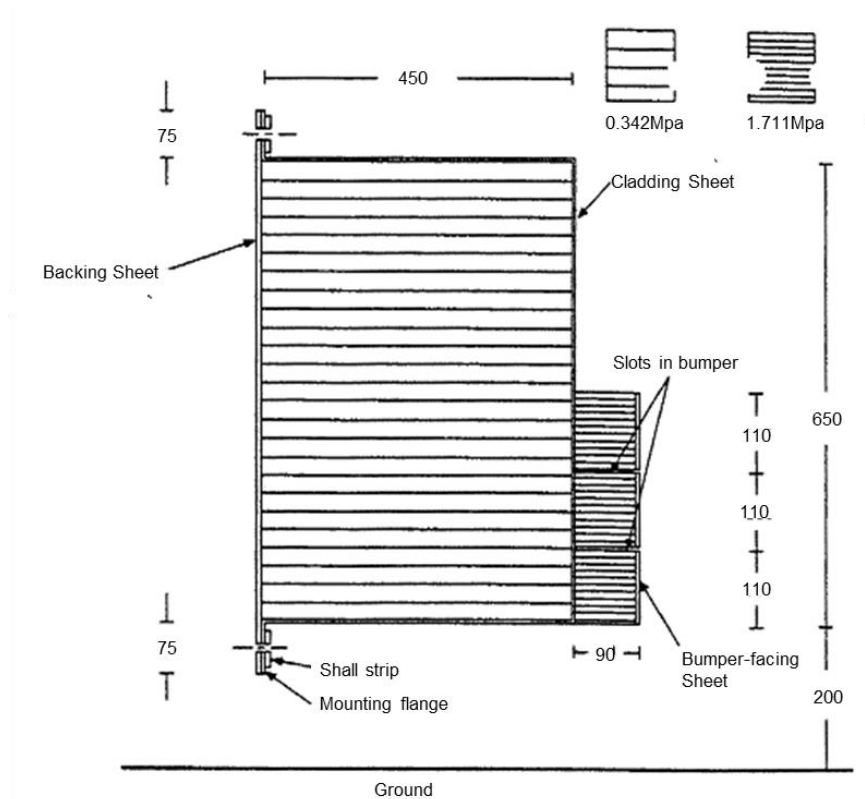
Figure 1: Deformable Barrier for Frontal Impact Testing
