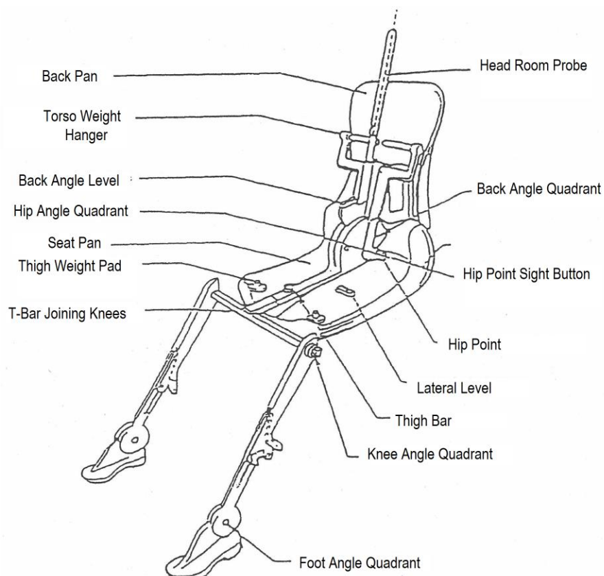
Figure 1 3-D Manikin Elements Designation
