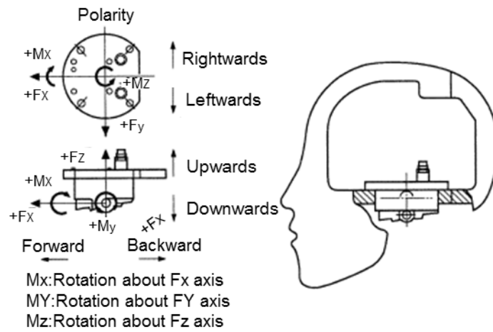
Figure 11: Installation of 6-axis Type Head Load Meter
