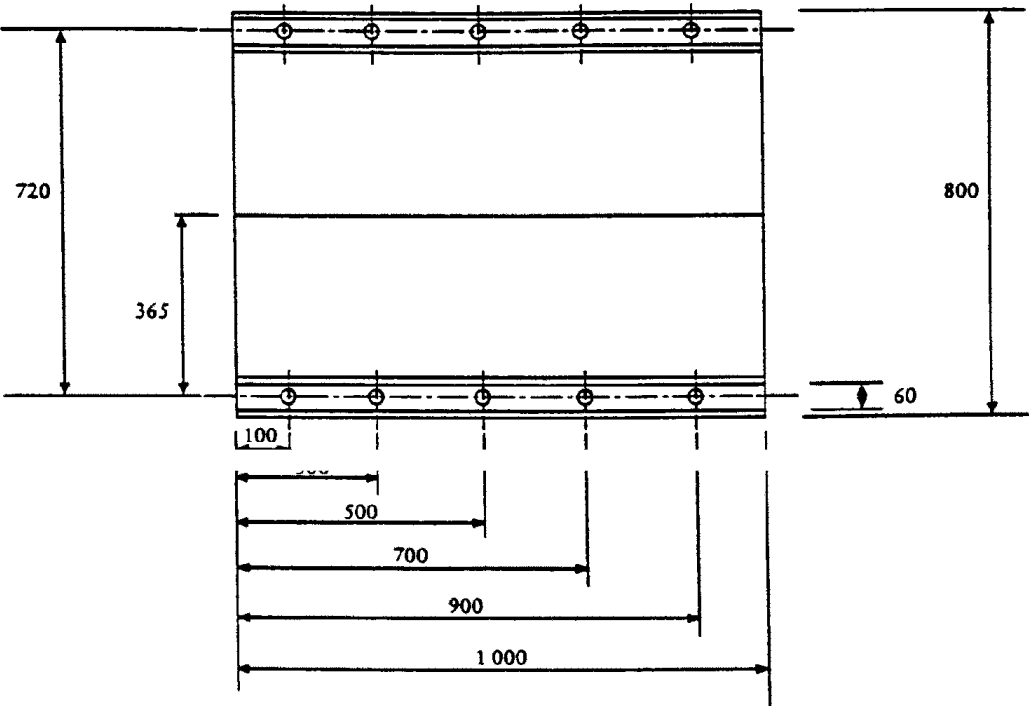
Figure 5: Positions of Holes for Barrier Mounting
