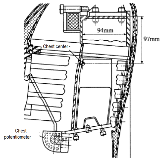
Figure 16 Center of Chest and Installation of Chest Potentiometer
