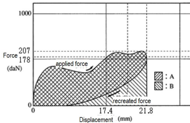
Figure 9: Chest Characteristics Test, Force-Displacement Curve
