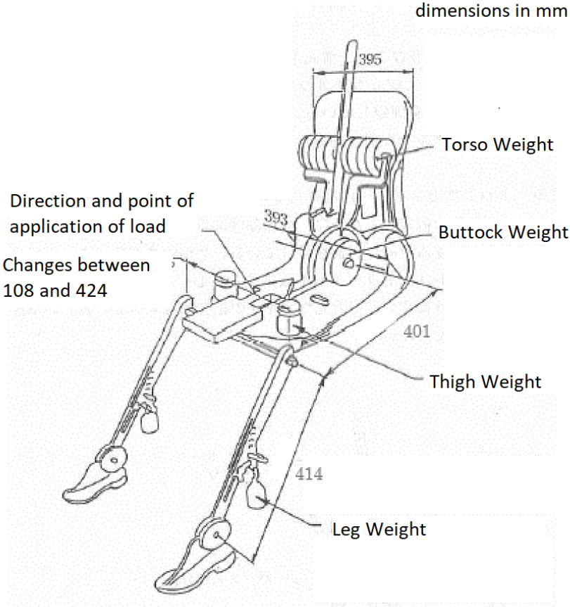
Figure 2 - Dimensions of the 3-D H Measuring Device Elements and Load Distribution
