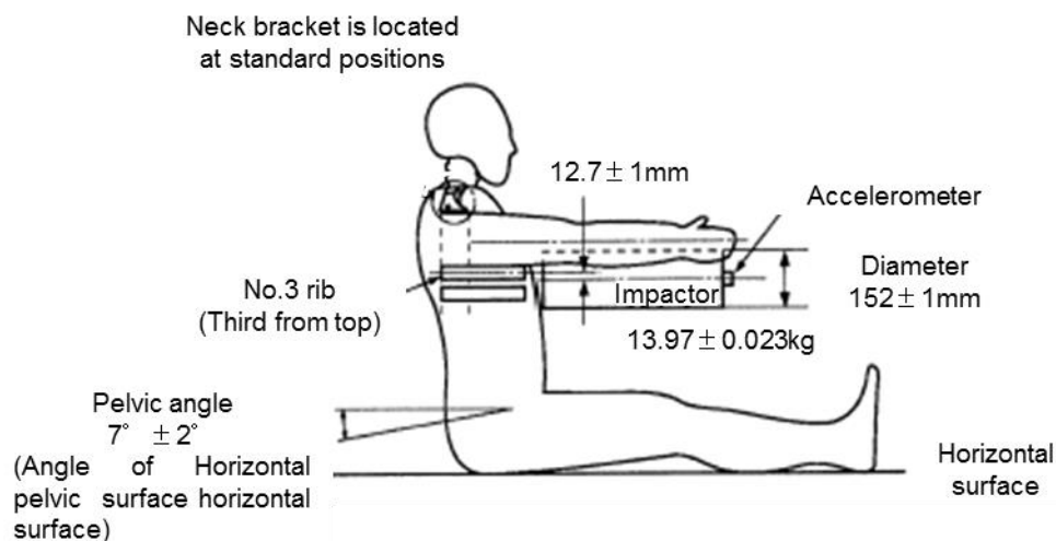
Figure 8: Chest Characteristics Test
