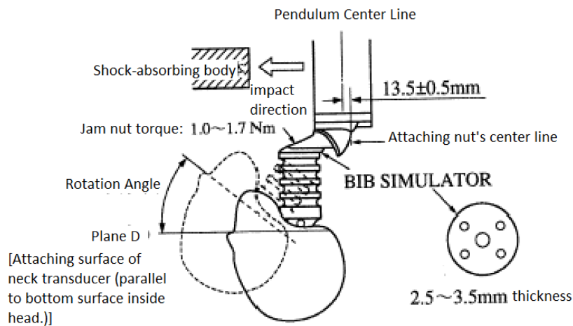
Figure 3: Neck Flexion Side Characteristics Test
