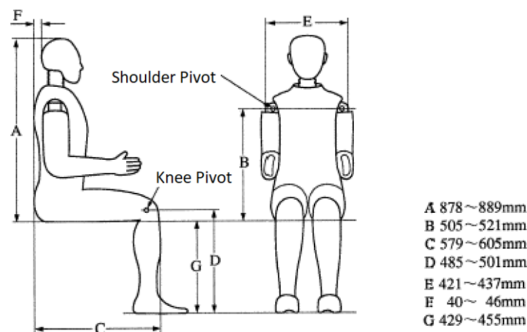
Figure 1: Hybrid III Mounting Dimensions
