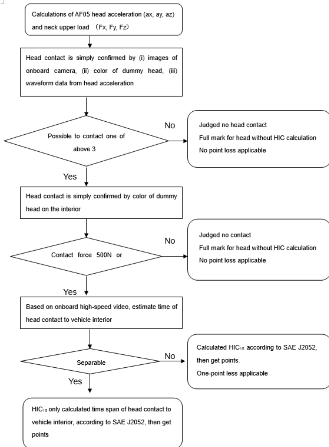
Figure 4: Secondary Head Collision Flowchart
