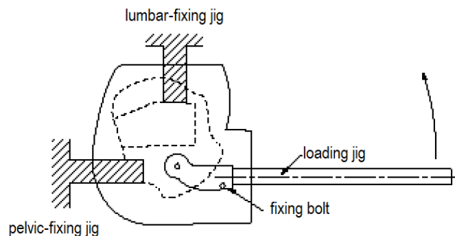
Figure 9: Bending Characteristic Test for the Upper Leg
