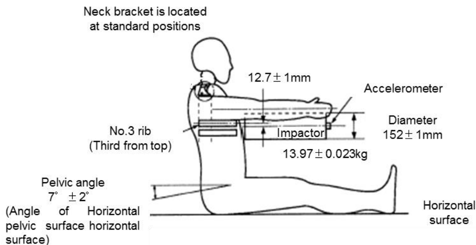
Figure 6: Chest Characteristics Test
