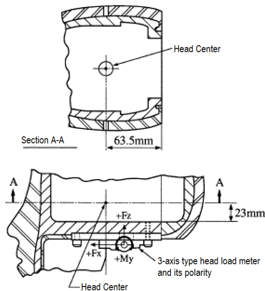
Figure 14: Center of Sensitivity of Head Accelerometer and Installation of 3-axis Type Head Load Meter
