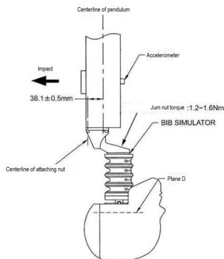
Figure 4 Neck Extension Side Characteristics Test
