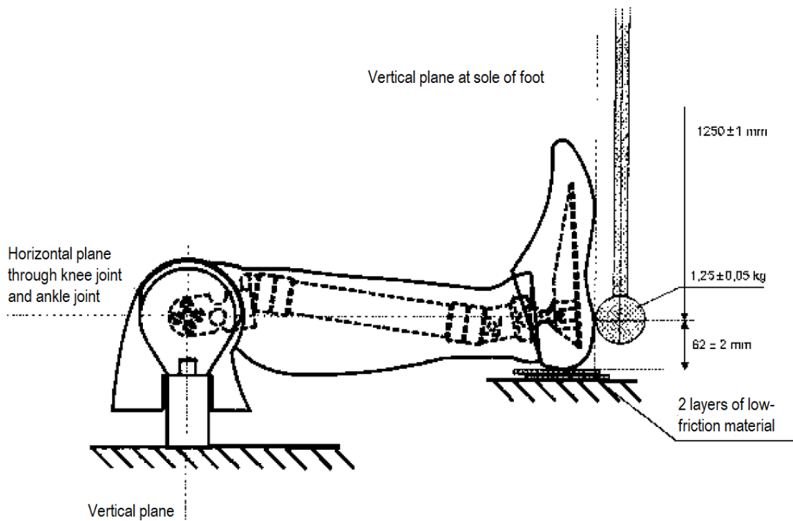
Figure 11: Lower Foot Impact Test (without shoe) (test set-up specifications)
