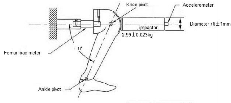
Figure 9: Leg Characteristics Test
