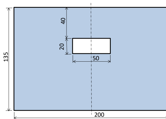
Figure 8: Secondary Collision Evaluation Range and Method for Opening a Through-Hole in the Dummy's Chest
