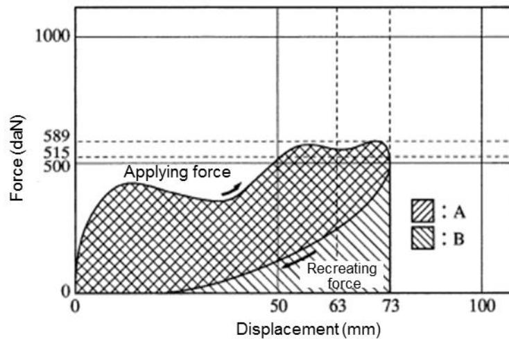
Figure 7: Chest Characteristics Test, Force-Displacement Curve
