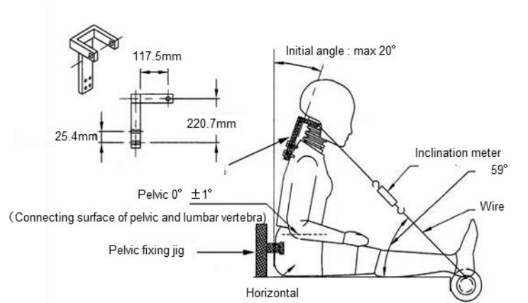
Figure 8 : Flexion Characteristic test for the Lumbar Vertebra
