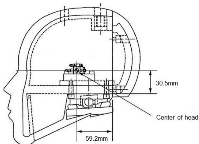
Figure 10: Head Accelerometer Sensitivity Center
