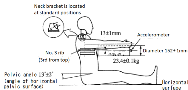
Figure 6 Chest Characteristics Test
