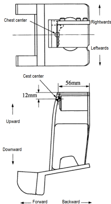
Figure 17: Center of Sensitivity of Chest Accelerometer
