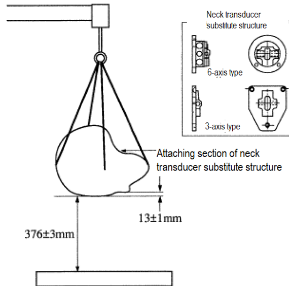
Figure 2: Head Characteristics Test
