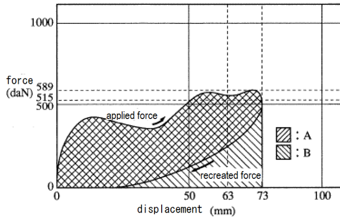
Figure 7 Chest Characteristics Test, Force-Displacement Curve
