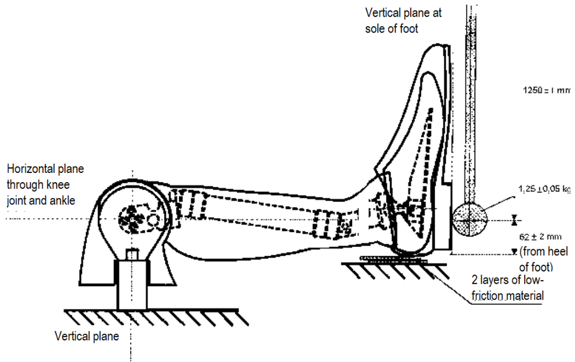
Figure 12 Lower Foot Impact Test (with shoe) (Test set-up specifications)
