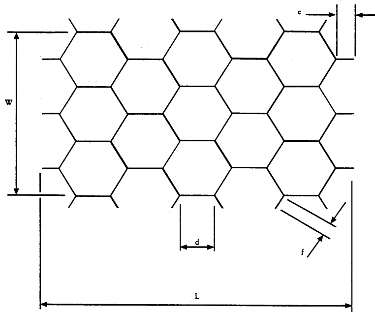
Figure 3: Honeycomb shaft and measurement dimensions
