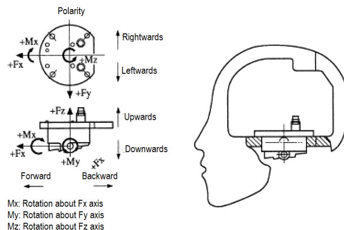
Figure 15: Installation of 6-axis Type Head Load Meter
