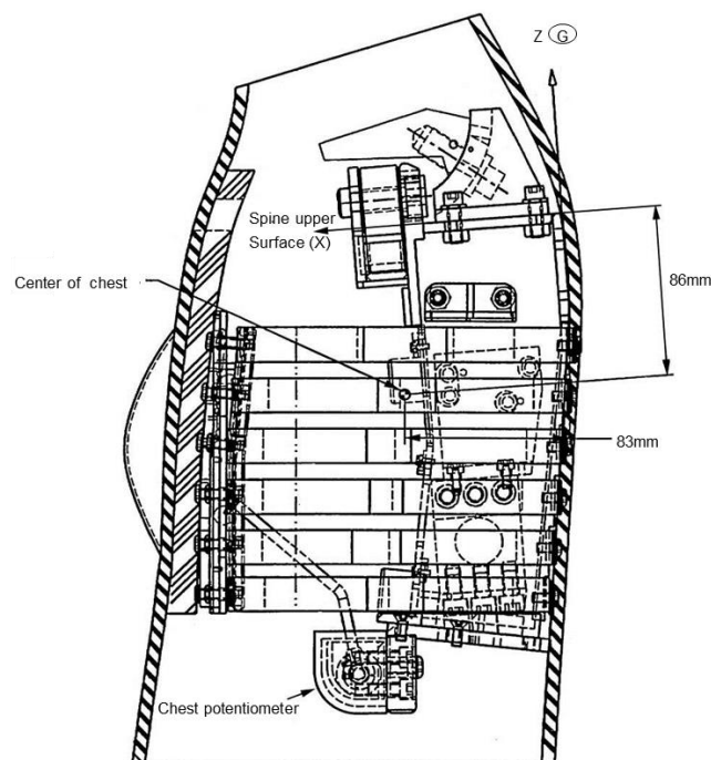
Figure 12: Center of Chest and Installation of Chest Potentiometer
