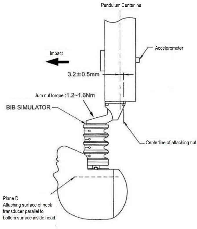
Figure 3. Neck Flexion Side Characteristics Test
