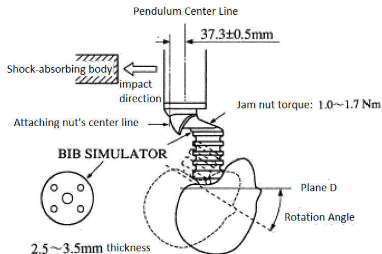
Figure 4: Neck Extension Side Characteristics Test
