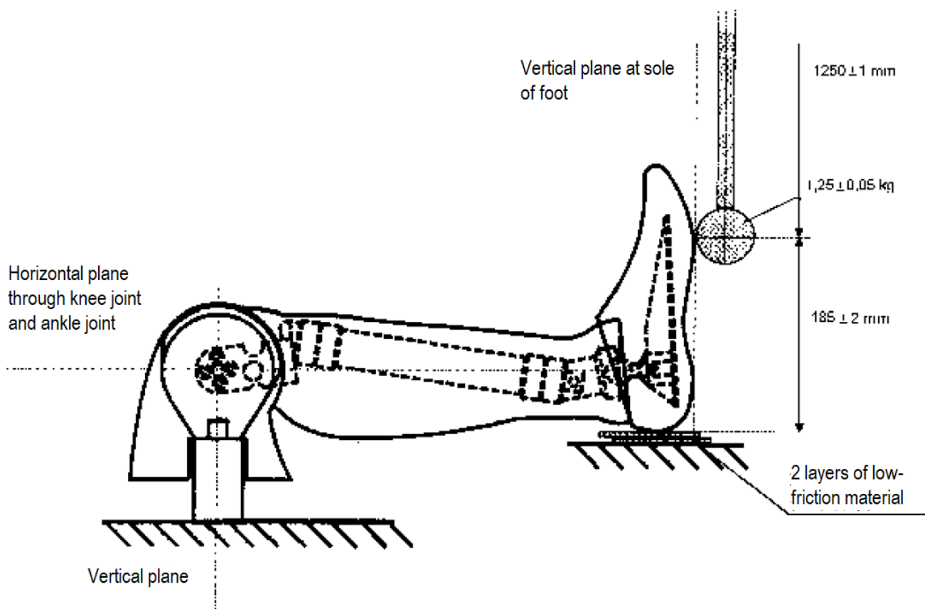
Figure 10: Upper Foot Impact Test (Test set-up specification)
